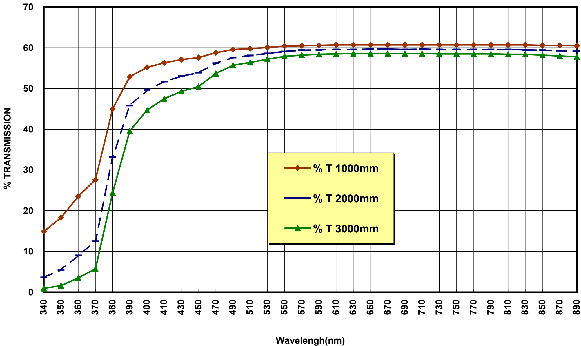
NA=0.55 FIBER BUNDLE TRANSMISSION, TYPICAL DATA
